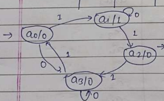
Moore Machine
